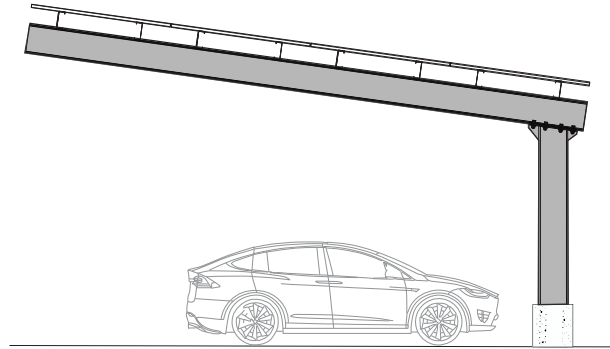
Full-Cant (HSSFC)
